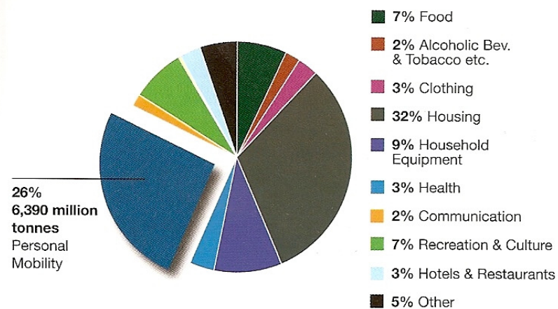
Figure 5.1: Personal Mobility's Global CO 2 Emissions
